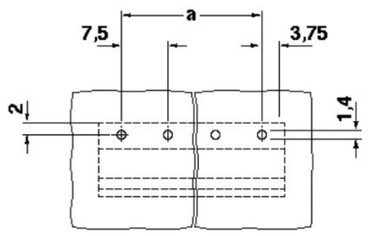
Drilling diagram
